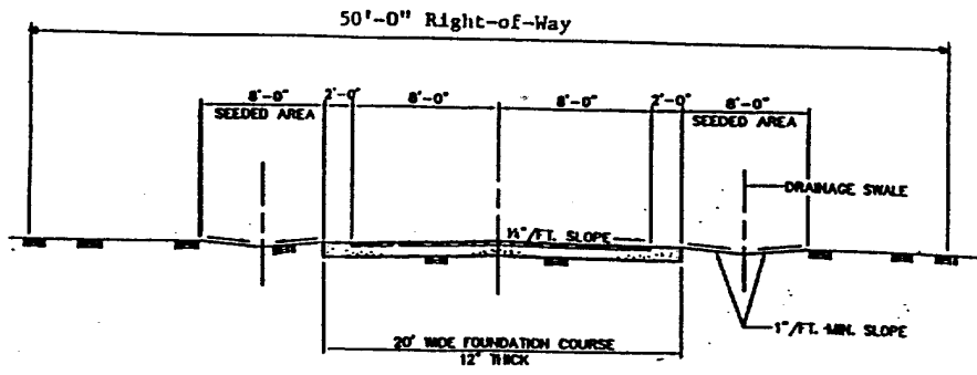
TYPICAL SECTION -- GRAVEL
